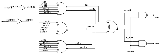
Figure 4: Hybrid CMOS/DCVSPGB 9-bit parity checker.
