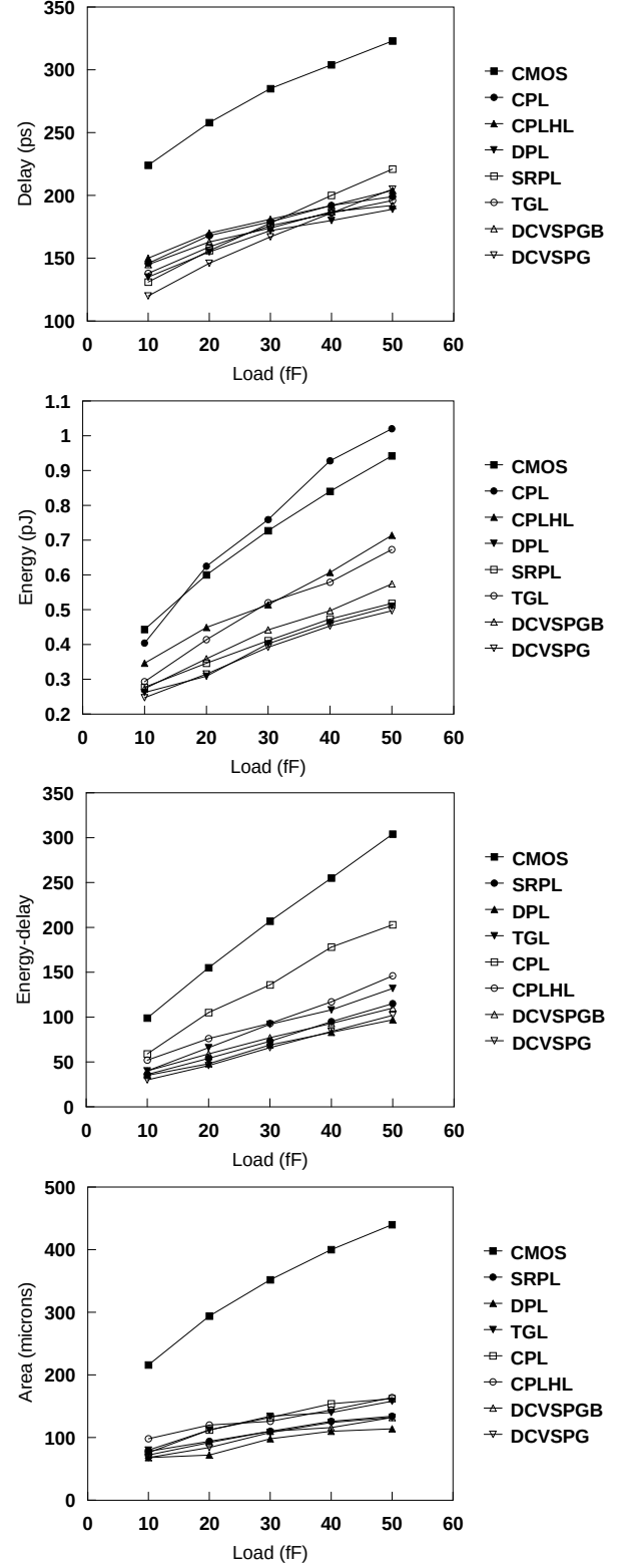
Figure 3: Results for delay, energy, energy-delay product and area for fixed-driver, variable-load experiment.
