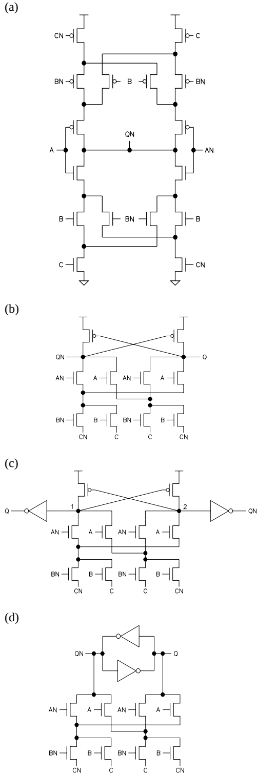
Figure 1: CMOS (a), DCVSPG (b), DCVSPGB (c) and SRPL (d) 3-input XOR gates used in experiment.
