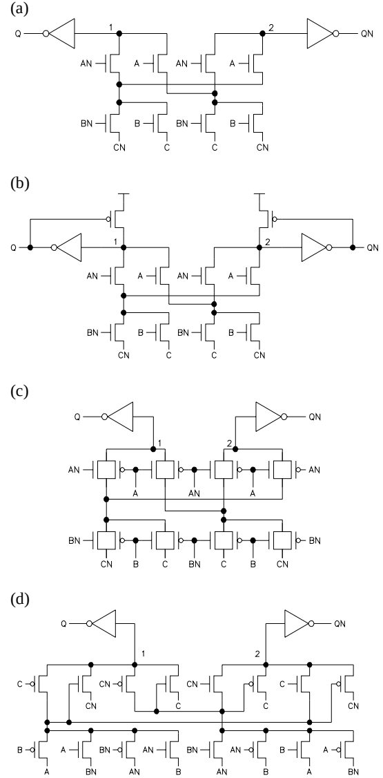
Figure 2: CPL (a), CPLHL (b), TGL (c) and DPL (d) 3-input XOR gates used in experiment.
