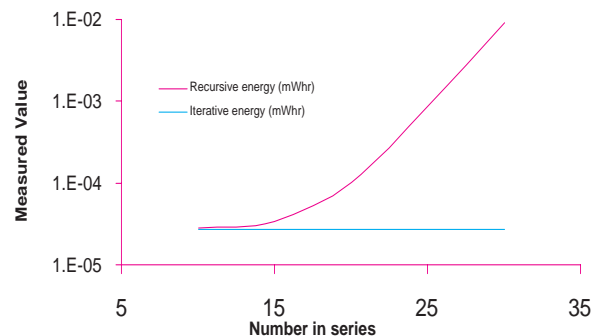
Figure 3: Energy Consumption of Recursive and Iterative Fibonacci
