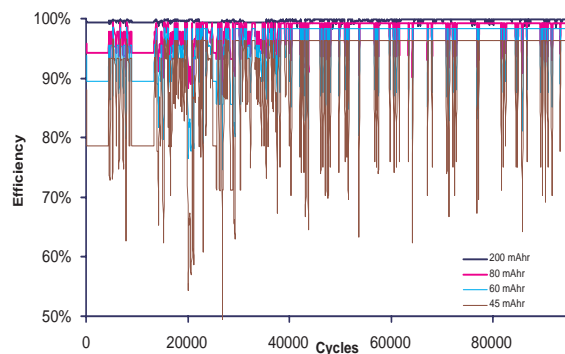
Figure 5: Battery Efficiency for MPEG Decoder
