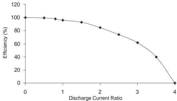
Figure 4: Battery Efficiency
