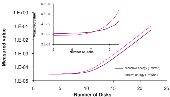
Figure 2: Energy Consumption of Recursive and Iterative Hanoi
