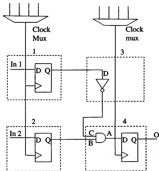
Figure 3. Example circuit for backtracing.
