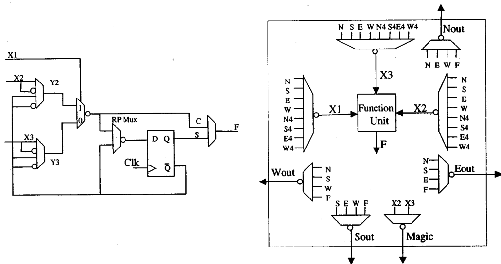
Figure 4. XC6200 Function Unit and Cell Routings.
