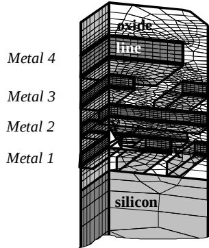
Figure 8. Densely packed 3-D interconnect array in a quadruple level metallization process. Self-heating of any line within such an array is strongly affected by the activity ( hot or cold ) of the neighboring lines.
