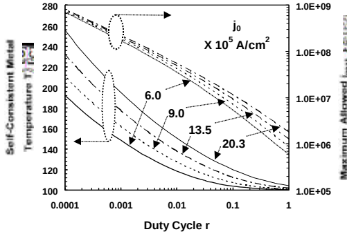
Figure 3. Self-consistent analysis showing dependence of T_m and j_{peak} on j_0 . Parameters used here are: t_{ox} = 3.0 \text{ } \mu\text{m} , t_m = 0.5 \text{ } \mu\text{m} , and W_m = 3.0 \text{ } \mu\text{m} . Interconnect metal is Cu.
