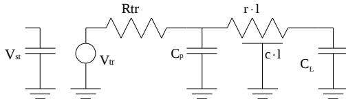
Figure 6. Equivalent distributed network for driver and interconnect. V_{st} is the voltage at the input capacitance that controls the voltage source. R_{tr} is the driver transistor resistance and C_L is the load capacitance of the next stage. l is the interconnect length.
