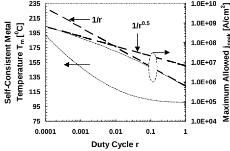
Figure 2. Self-consistent solutions for T_m and j_{peak} . Parameters used here are: j_0 = 0.6 \text{ MA/cm}^2 , t_{ox} = 3 \text{ } \mu\text{m} , t_m = 0.5 \text{ } \mu\text{m} , and W_m = 3 \text{ } \mu\text{m} . Interconnect metal is Cu with \rho_m(T_m) = 1.67 \times 10^{-6} \Omega\text{-cm} [1 + 6.8 \times 10^{-3} (T_m - T_{ref})] . The two dotted lines indicate j_{peak} values based on a) j_{peak} = j_0/r , and b) j_{peak} = j_{rms}/r^{0.5} .
