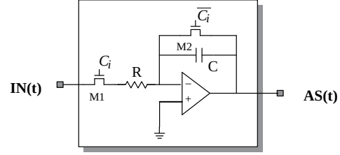
Figure 1: Analog signature analyzer
