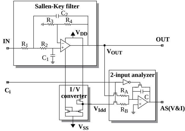
Figure 5: Mixed voltage/current signature
