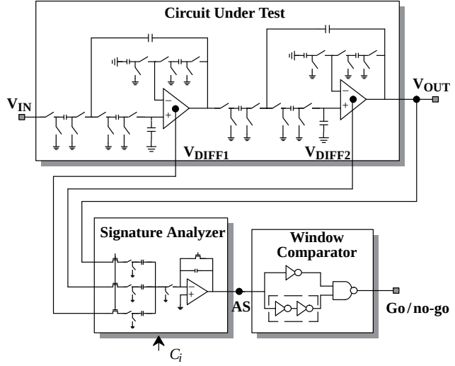
Figure 6: Self-testing switched-capacitor filter
