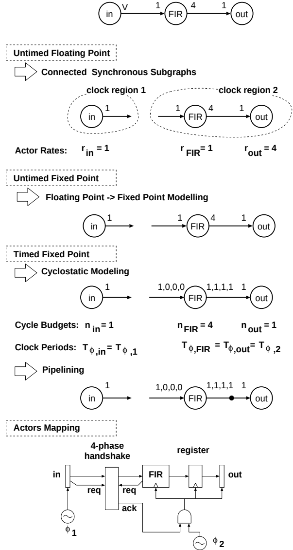
Figure 4: Refinement flow
