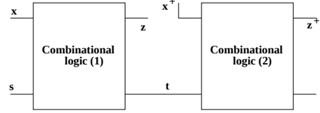
Figure 3: Unrolling of a FSM.
