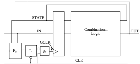
Figure 5: Modified Gated-Clock Architecture.
