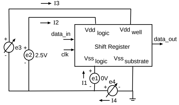
Fig. 4: Circuit simulation of the shift register.
