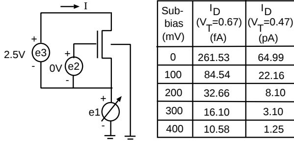
Fig. 3: Simulation of sub-threshold slope for an NMOS transistor.
