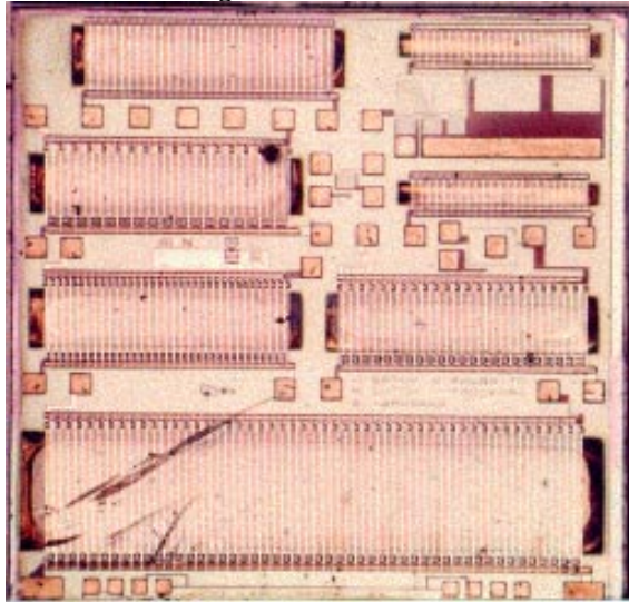
Figure 6: Fabricated micro-fluxgate sensing element [Kaw95]
