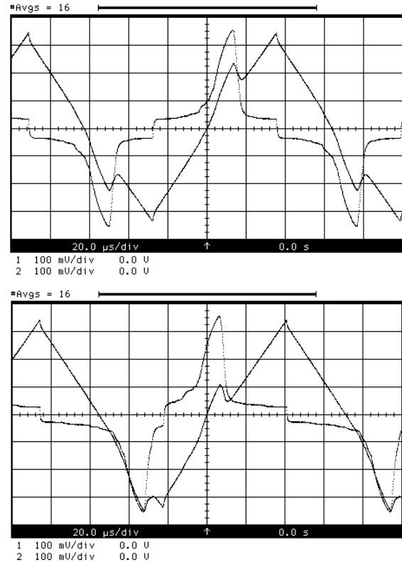
Figure 4: Real fluxgate sensor data, without and with a field applied.
