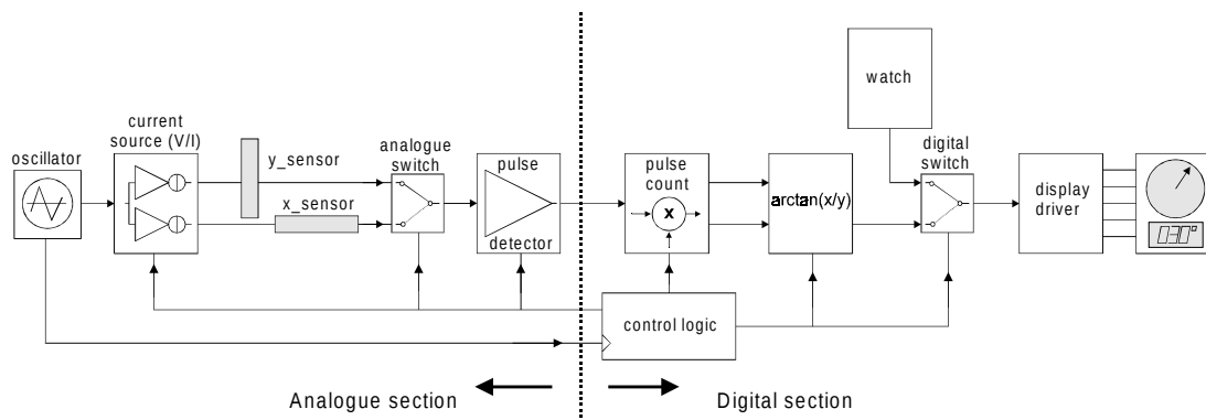
Figure 1: Overview of the electronic compass system
