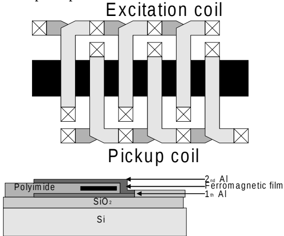
Figure 5 : Structure of the fluxgate sensing element
