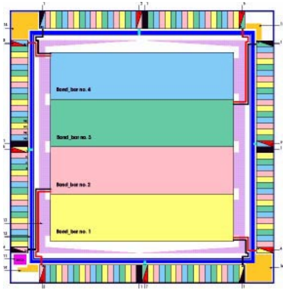
Figure 2: The fishbone Sea-of-Gates Array
