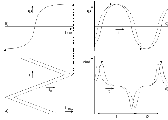
Figure 3: Pulse position operating principle of a fluxgate sensor, H_{exc} \equiv I_{exc} and V_{ind} = d\Phi/dt
