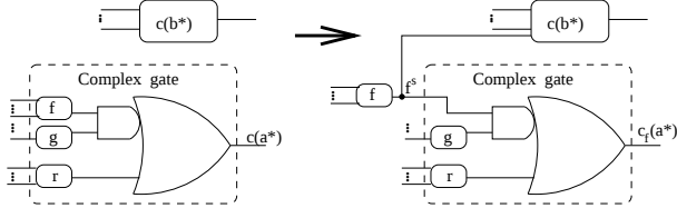
Figure 4: Decomposition of the cover function c(a^*)
