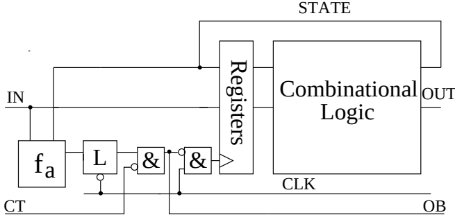
Figure 5: Gated-clock FSM with increased controllability and observability.
