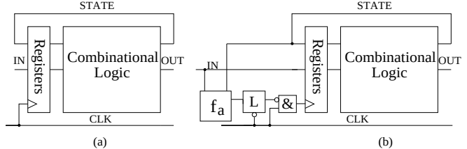
Figure 1: (a) Single clock, flip-flop based finite-state machine. (b) Gated clock version.
