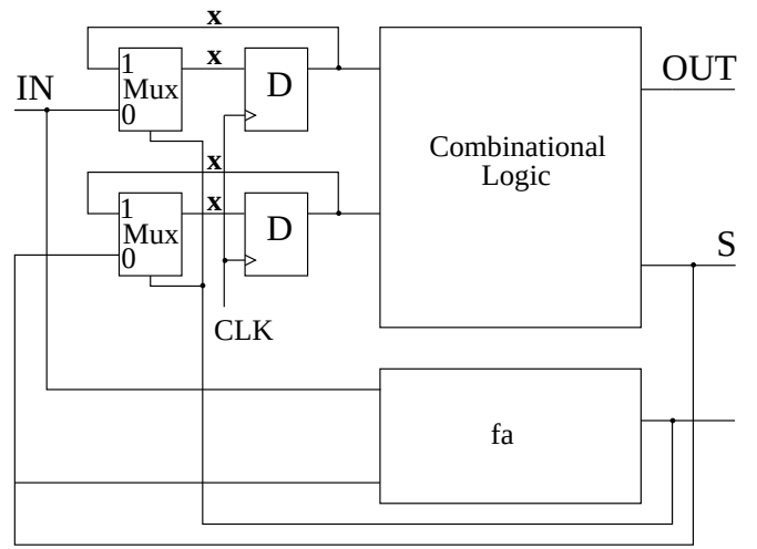
Figure 3: Multiplexed model of a gated-clock FSM.
