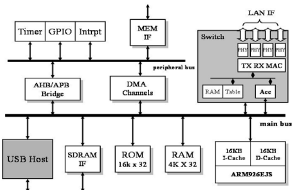
Figure 4. SoC platform
