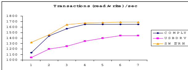
Figure 8. Varying SDRAM OO queue size
