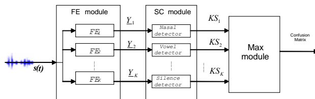
Knowledge Extraction Module, adapted from [6]. The detectors are based on a MLP neural network.
