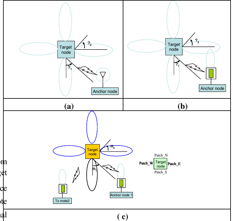
Figure 7. Antenna configurations for (a) Experiment 1 (b) Experiment 2 (c) Experiment 3
