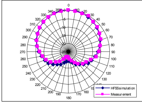
Figure 6. Radiation pattern of the patch antenna from HFSS and the measurement in anechoic chamber room
