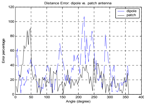
Figure 8. Relative error in distance estimation for Experiment 1
