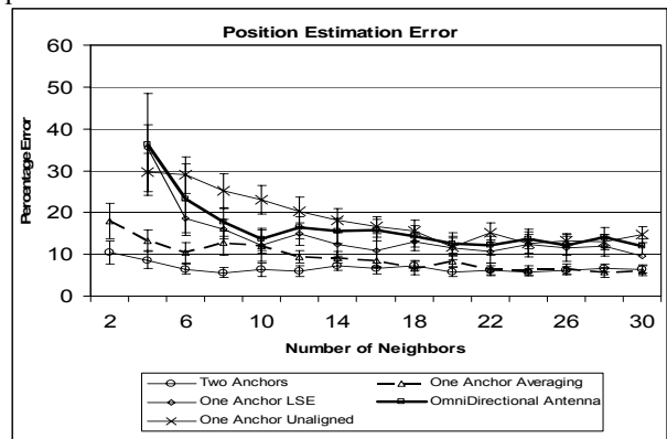
Figure 13. Evaluation of estimation error for varying number of neighboring anchors
