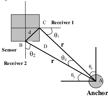
Figure 3. Location determination with an omnidirectional transmitter and directional receiver
