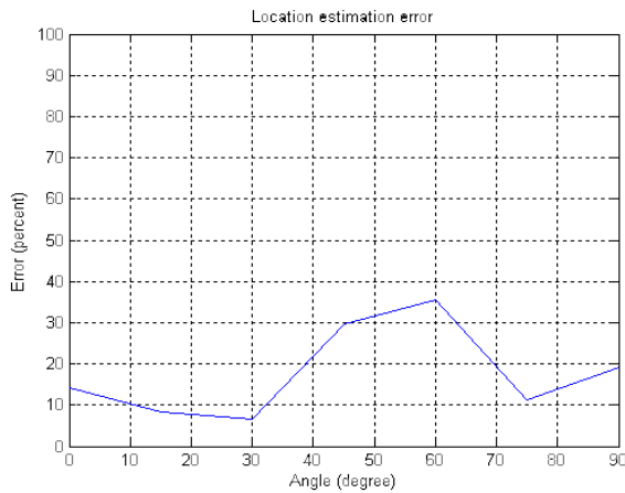
Figure 12. Location estimation error for two anchor nodes with directional patch antennas
