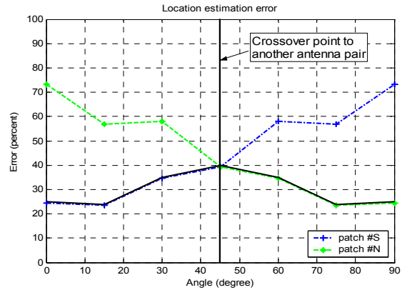
Figure 11. Location estimation error for Experiment 2
