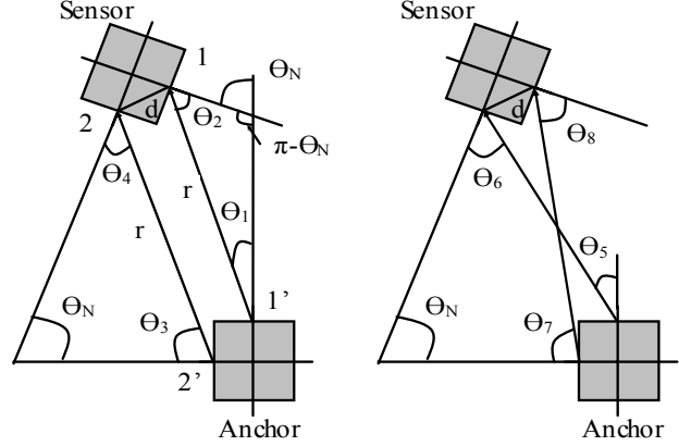
Figure 4. Location determination for unaligned antennas
