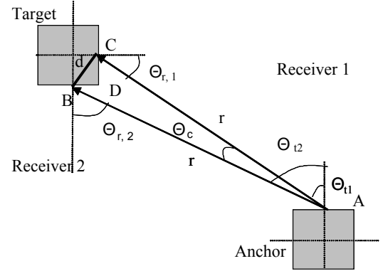
Figure 2. Location determination with aligned nodes
