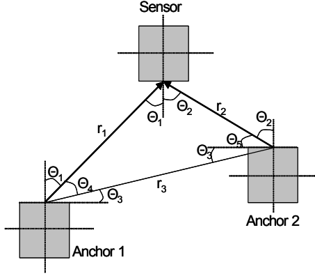
Figure 5. Location determination using measurements from two anchors
