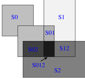
Figure 4. Subscription rectangles at leaf servers
