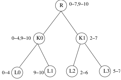
Figure 1. Pub/sub tree
