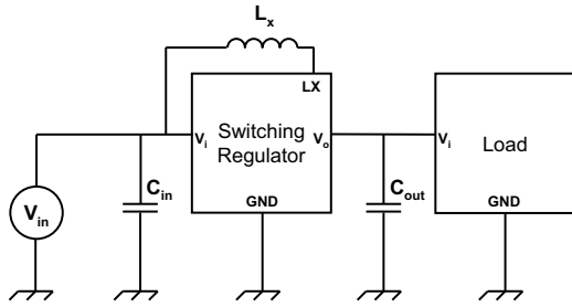
Figure 1. A typical system with switching regulator-based power supply, including the regulator, input capacitor, output capacitor, inductor, and load.
