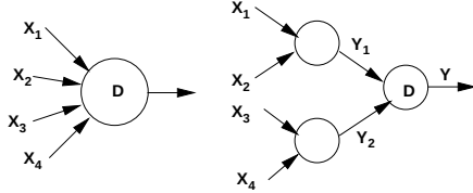
Figure 3: Reducing the Maximum Fanin in the DAG
