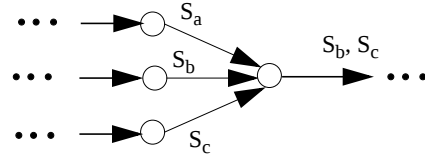
Figure 5. Propagation of required times.
