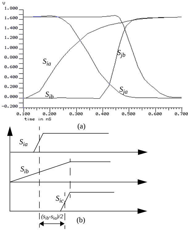
Figure 4. Bound on added path delay
