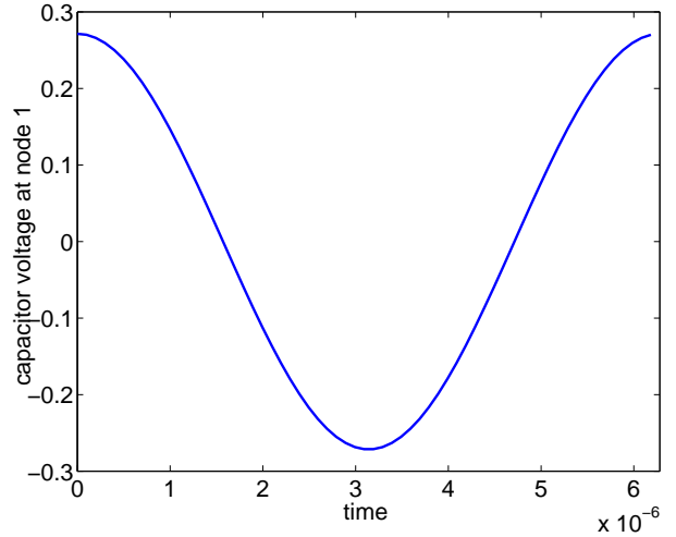
Figure 1: Oscillator steady-state: voltage at capacitor
