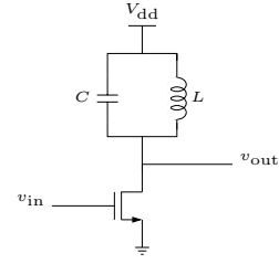
Figure 7: LC resonator.
