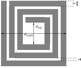
Figure 1: Square inductor layout and geometry.
