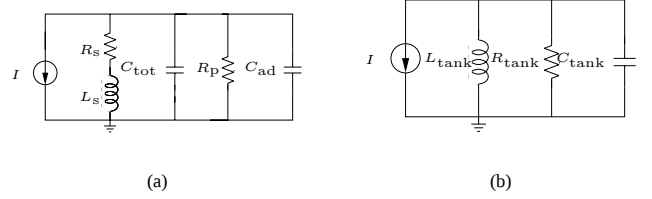
Figure 8: LC resonator small-signal circuit
