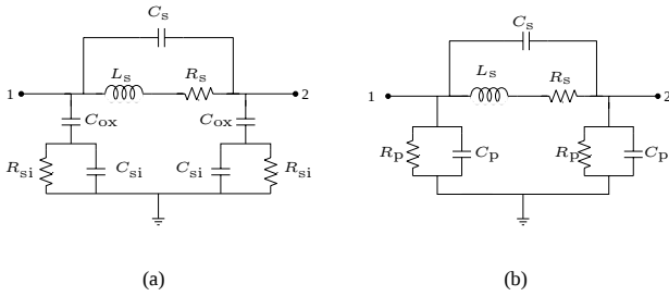
Figure 2: Inductor model: (a) \Pi model, (b) simplified model.
