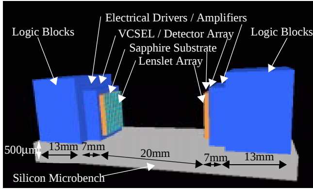
Figure 4: FFT Optical MEM System
