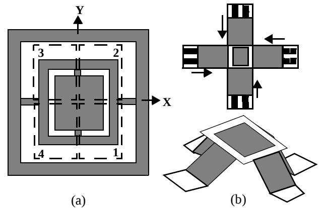
Figure 8: (a) Scanning Mirror and (b) MESA Structure[11]
