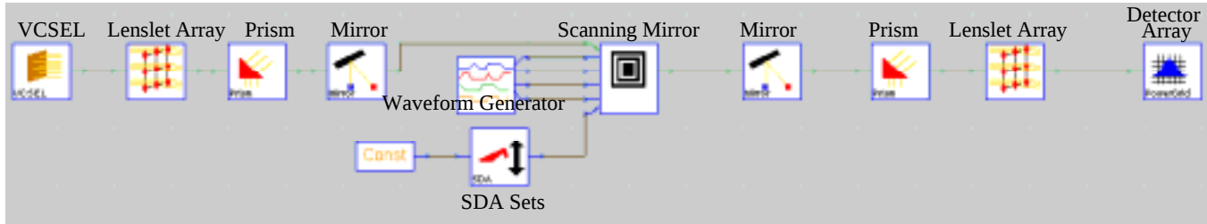
Figure 9: Scanning Mirror System in Chatoyant
