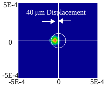
Figure 5: Intensity distributions of a 1\text{ }\mu\text{m} VCSEL Offset Propagated 20mm to the Second Lenslet Array
