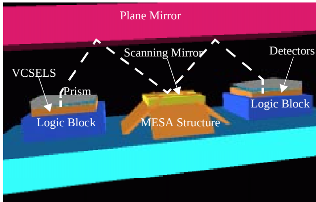
Figure 7: Other system using optical MEM scanning mirror
