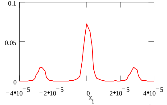
Figure 6: Scalar Intensity Distribution at the 80\text{ }\mu\text{m} Detector
