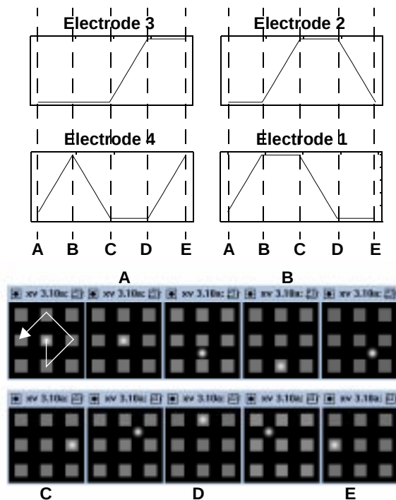
Figure 10: Waveforms and Snapshots of Scanning Pattern
