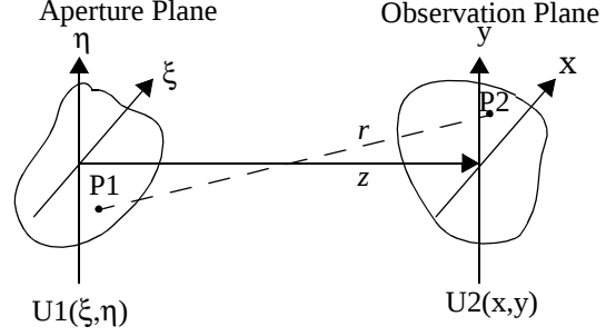
Figure 1: Diffraction Geometry for Fresnel and Fraunhofer Approximations
