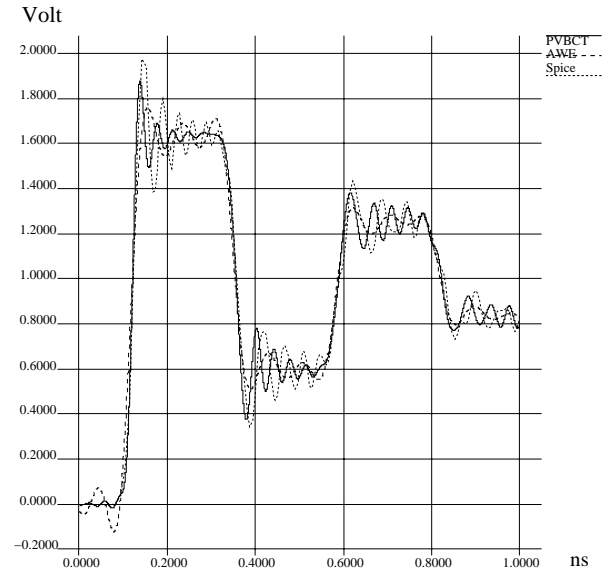
Figure 6: RLC circuit simulation result.
