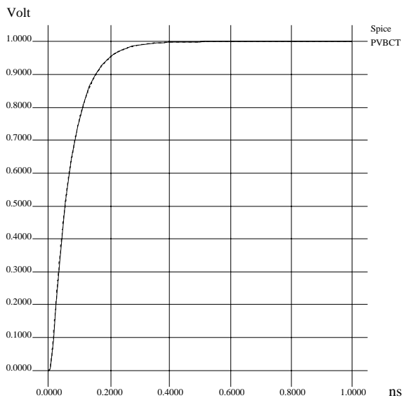
Figure 8: RC circuit simulation result.
