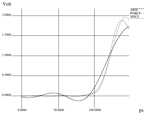
Figure 7: Enlarged RLC circuit simulation result.
