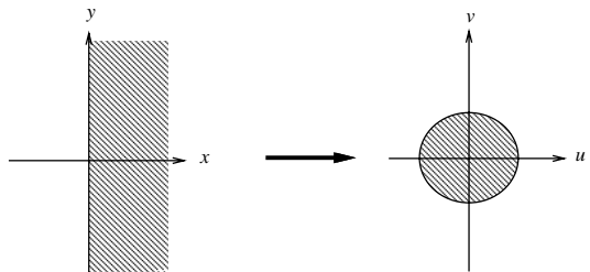
Figure 2: The conformal transformation \frac{1-z}{1+z} .
