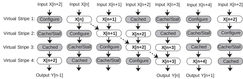
Figure 15: Example of the data flow for the broadcast convolution. The configuration controller inserts stalls to reduce bus contention(which cause the virtual stripes to remain cached longer). The dashed lines indicate how Y[n] is accumulated as time progresses.
