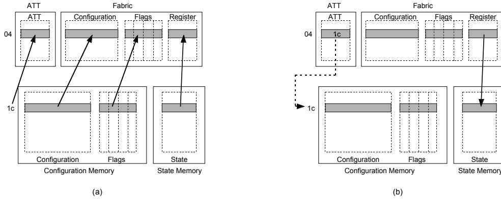
Figure 10: Restoring (a) and storing (b) state between fabric, configuration memory, state memory and ATT.
