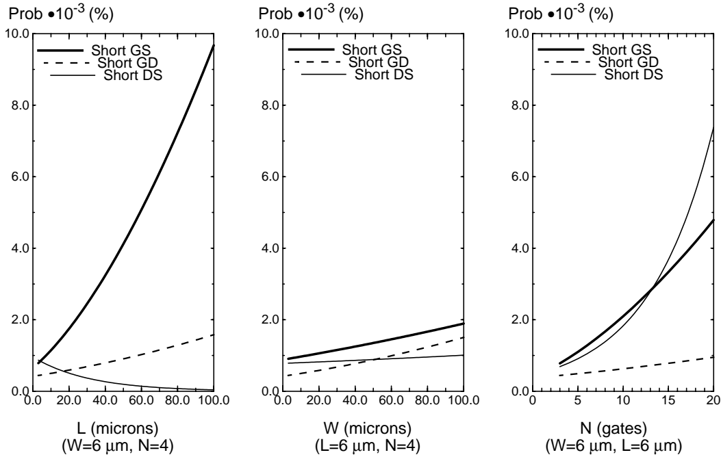
Fig. 4: Predicted probabilities of shorts for interdigit transistors
