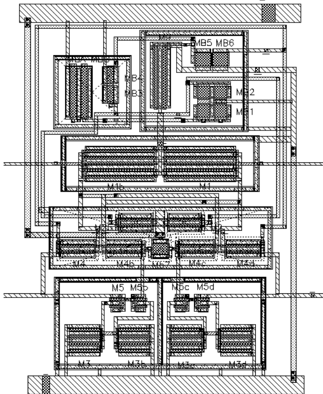
Fig. 6: Layout of the fully-differential opamp
