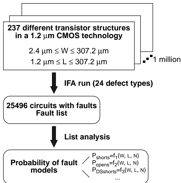
Fig. 1: Model derivation flow
