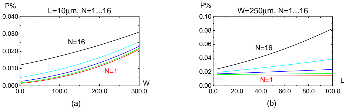
Fig. 3: Probability of faults given by the Level 1 model for transistors with: (a) L=10\mu\text{m} , (b) W=250\mu\text{m} .
