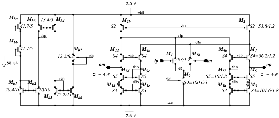
Fig. 5: Fully-differential operational amplifier
