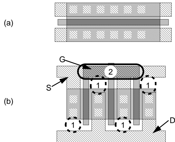
Fig. 2: Different transistor shapes: (a) rectangular, (b) interdigit.
