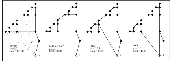
Figure 5: Example where the performance ratio of BPRIM is not bounded for any \epsilon
