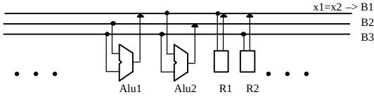
Fig. 5.b: Impact on interconnect generation
