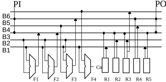
Fig. 7.b Interconnect network with test constraints
