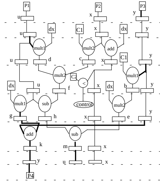
Fig. 2: Scheduled data flow graph
