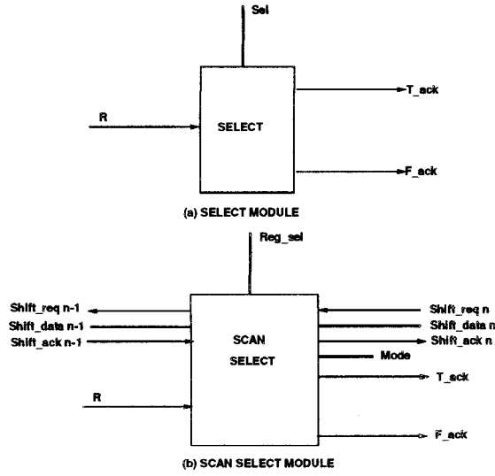
Figure 4: Interface of SELECT and SCANSELECT modules
