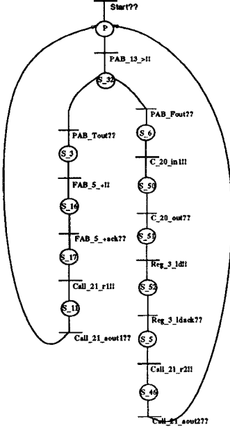
Figure 2: NHFG for the example
