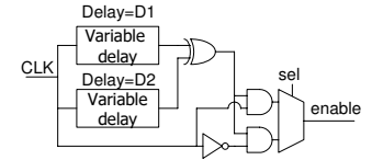
Fig. 4. Circuit for ‘enable’ signal generation.
