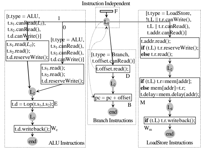
Figure 5- RCPN sub-nets
