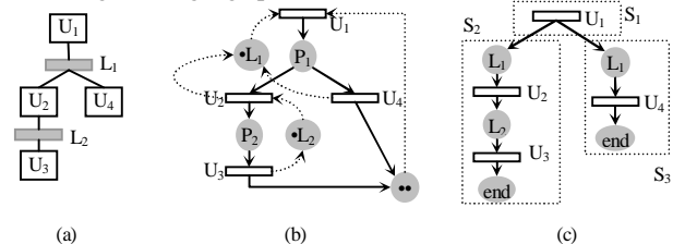
Figure 2- An Example Pipeline structure(a) and its CPN(b) and RCPN(c) models
