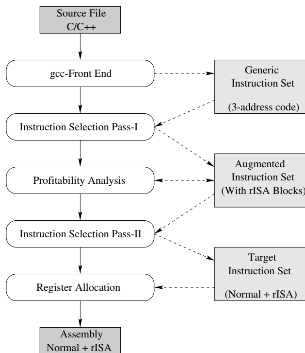
Figure 1. EXPRESS compiler flow
