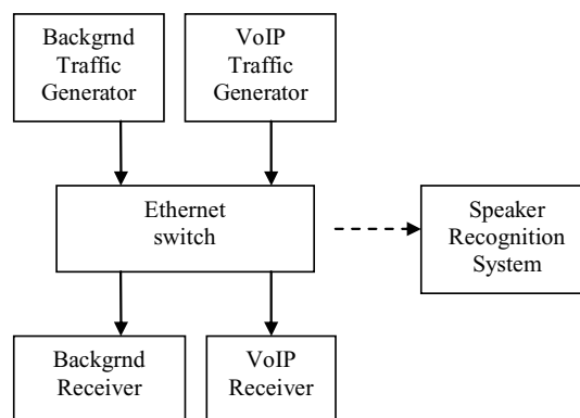
Figure 6: Experimental testbed
