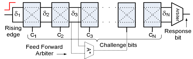
Fig. 1. Parallel PUF structure. The feed forward arbiter (shown in the dashed line) is used to introduce nonlinearity.
